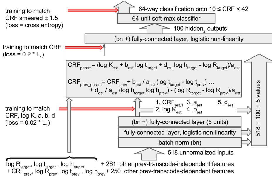
Figure 8: Layout of neural network used to estimate, when a previous transcode is available
