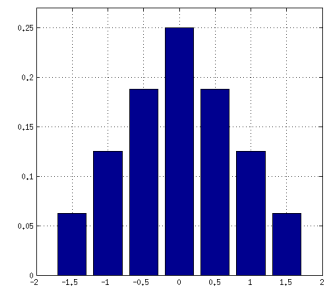
Figure 6: Label smearing used for going from actual CRF of the transcode to a multi-class label. By smearing over \pm 1.5 CRF units, we lessen the categorization penalty for bitrate errors that are less than 20%
